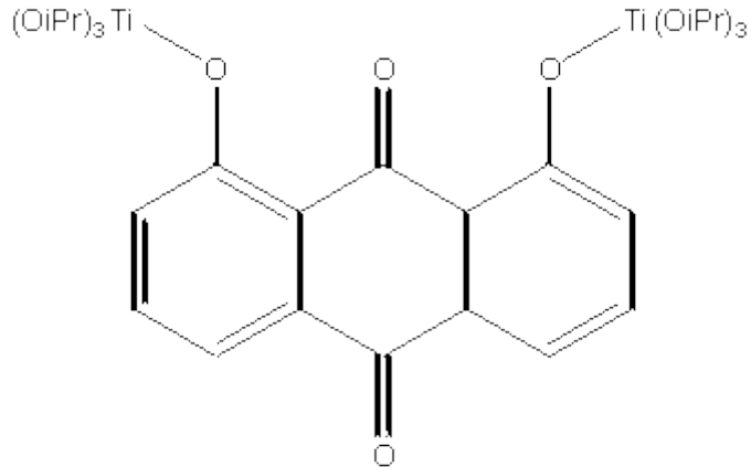
Lewis Acid
