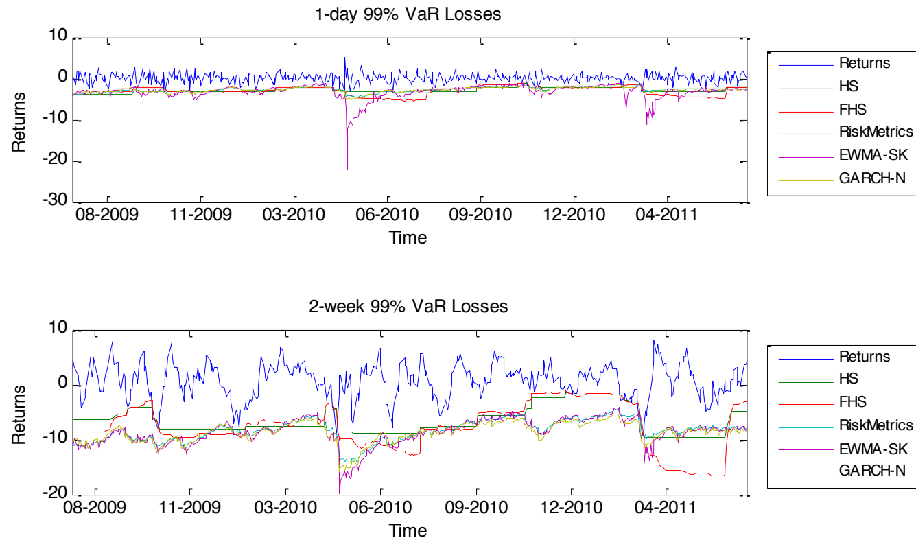
Figure 8: Out-of-sample 1-day and 10-days volatility forecasts and 99% VaR losses of the DAX 30 equity index
