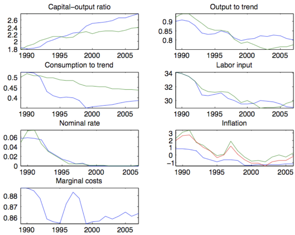
Figure 2: Baseline economy
