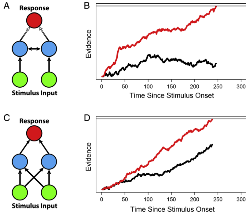
Fig. 1. Graphical depiction of models compared. The top row (i.e., Panels A and B) corresponds to the LCA model, whereas the bottom row (i.e., Panels C and D) corresponds to the FFI model. The left column (i.e., Panels A and C) shows a graphical representation of how the stimulus input is mapped to the behavioral response. The right column (i.e., Panels B and D) shows a representative simulation of each corresponding model in a two-alternative decision task.
