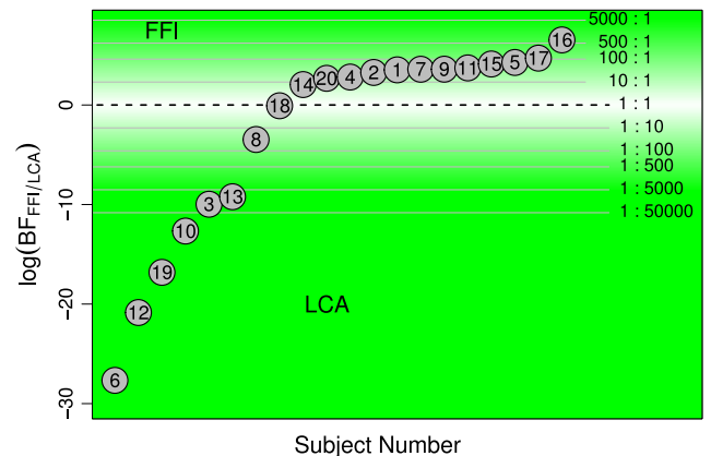
Fig. 2. The Bayes factors comparing the FFI model to the LCA model for each subject. Subjects have been ranked in increasing order, where a higher Bayes factor corresponds to greater evidence for the FFI model. The point of indifference between the two models is represented as the dashed horizontal line at zero.
