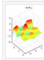
Figure 1: A numerical solution of (4.1) with E = 5 (in units adopted throughout the paper), R_H = 3/5 , and A_2 \equiv 0 . The initial values \psi_2(x, 0) = 0.3 \exp(ix) + 0.2 * \exp(2ix) , \psi_1(x, 0) = -0.9 \psi_2(x, 0) , and A_1(x, 0) = 0 are prescribed on the edge facing front right.
