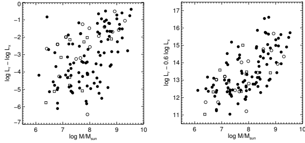
Fig. 4. The left panel shows the logarithm of the ratio of radio to X-ray luminosity, \log L_R - \log L_X vs. the logarithm of black hole mass for the SMBH in the sample. The right panel shows instead the ratio L_R/L_X^{0.6} . The latter shows clearly a stronger correlation with black hole mass than the former. Note that this plot removes the distance bias up to the level that black hole mass is only very slightly correlated with distance within the extragalactic SMBH sample (this can be seen from Figure 3). Open symbols are upper limits.
