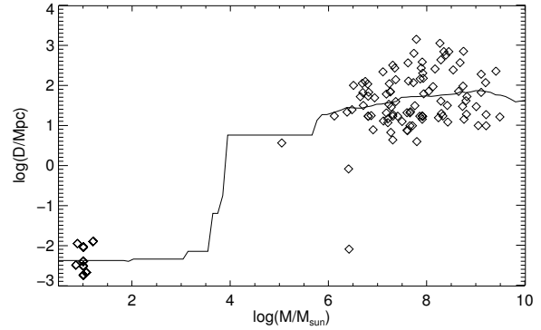
Fig. 3. Distance vs. black hole mass for the objects in the MHD03 sample. the solid line is the sliding mean. This shows that the AGN sample is homogeneous in distance with mass and therefore any L_R/L_X^{\xi_{RX}} vs. M relation in the AGN sample cannot be driven by distance.
