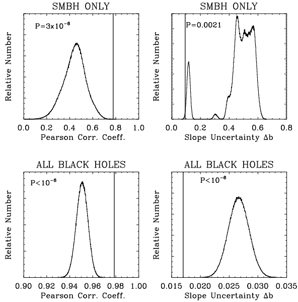
Fig. 2. Results of the Monte Carlo simulation of scrambled radio fluxes. Upper panels : extragalactic supermassive black holes only; lower panels : entire sample of detected sources, including XRBs; left hand panels : distributions of the Pearson’s correlation coefficients for randomized fluxes (curve), compared to correlation coefficient of the original dataset (vertical line) — larger is better; right hand panels : distributions of the uncertainties in the regression slope for the randomized fluxes (curve), compared to the value for the original data (vertical line) — smaller is better. Also shown are the Monte Carlo likelihoods for the observed values as random chance realizations of the randomized sample (upper left corners). All plots show clearly that the randomized sample is not as strongly correlated as the real one.
