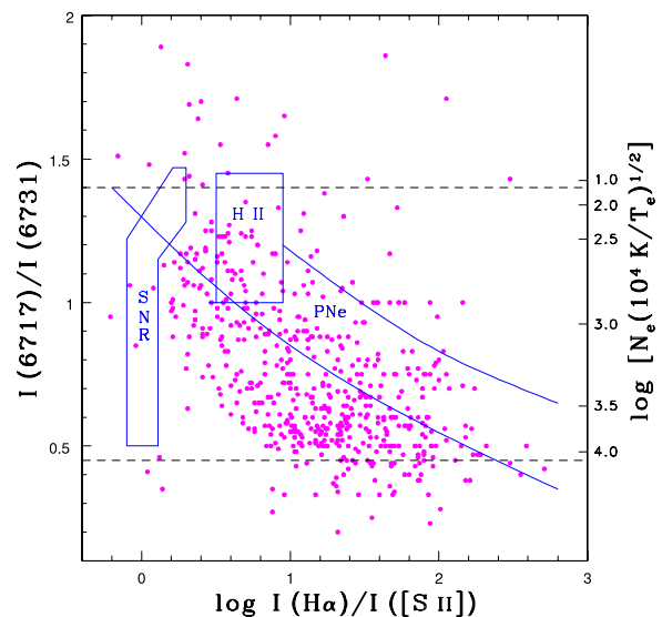
Fig. 2. As in Figure 1, but for the \log [H\alpha/[S II]] versus [S II] \lambda\lambda 6717/6731 plane. The horizontal dashed lines indicate the range of values for which the [S II] \lambda\lambda 6717/6731 ratio is a valid indicator of the electron density.
