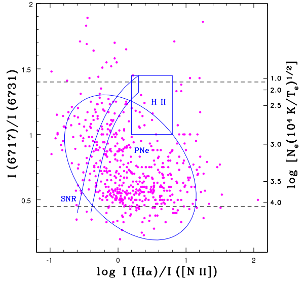
Fig. 6. As in Figure 4, but for the \log [H\alpha/[N II]] versus [S II] \lambda\lambda 6717/6731 plane. The correlation coefficient is -0.37 .
