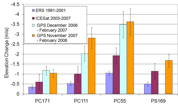
Fig. 2. Rates of elevation change from GPS measurements, laser altimetry (Appendix A) and radar altimetry (Shepherd et al., 2002).
