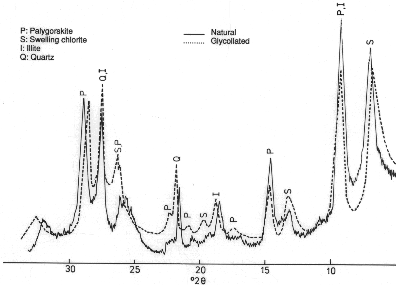
Figure 1. XRD traces of glycollated and unglycollated samples of palygorskite-bearing clay from Edith Creek. CuKα radiation
