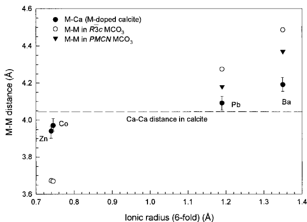
FIGURE 12. Observed M-Ca distances (solid circles) in the synthetic M-doped calcites plotted as a function of ionic radius of the impurity M. Open circles are the corresponding M-M distances in the pure \text{MCO}_3 compounds with the calcite structure ( R\bar{3}c ); values for \text{PbCO}_3 and \text{BaCO}_3 are extrapolated from the trend of known R\bar{3}c structures. The M-Ca distances are closer to the Ca-Ca distance in ideal calcite than to corresponding distances in their respective pure metal carbonates. Triangles give the shortest M-M distances in orthorhombic \text{PbCO}_3 and \text{BaCO}_3 , which fall between values in the rhombohedral structures.
