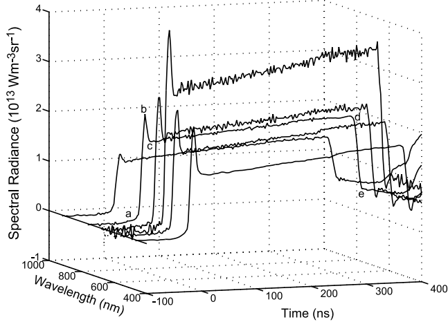
Figure 4. Representative time-resolved radiance profiles recorded by the six-channel pyrometer ( \text{MgSiO}_3 glass, shot 335). Times marked a – e correspond to key events discussed in text upon loading and unloading.
