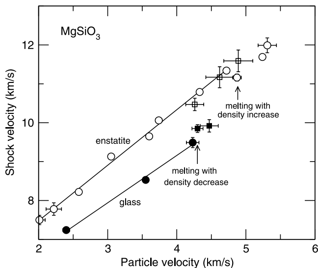
Figure 9. U_s - u_p relations for shocked \text{MgSiO}_3 glass and enstatite from this work (squares) and Akins [2003] (circles). Solid lines are linear fits in Pv regime beyond which Pv melts with positive (on glass Hugoniot) and negative (on enstatite Hugoniot) Clausius-Clapeyron slopes. Note that enstatite data from radiation history (open squares) agree with Akins [2003] within experimental uncertainties. In general, the uncertainties in U_s and u_p from radiation history are larger than those from streak-camera diagnostics as employed in Akins [2003]. (Some error bars are smaller than the symbol size.)
