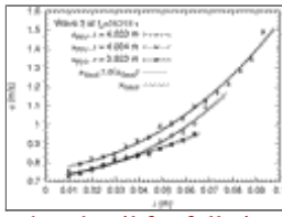
FIG. 3. Graphs of the PIV measured x velocities, u_{\text{PIV}} , with their standard deviations, along with the fitted x velocities, u_{\text{fitted}} , extrapolated to the positions of the fluid surface, \eta_{\text{PIV}} , for three values of x along Wave 3 at t_{\mathbf{v}} = 242/16 s. Note that the error bars are aligned horizontally in the key but vertically on the plot
