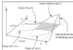
FIG. 1. Schematic diagram of the parameters used in the defining equation, Eq. (1), of the kinematic breaking criterion. The hatched region on the (x, t) -coordinate plane, x_d(t_U) < x < x_U , t_d(x_U) < t < t_U , is the region in which the criterion is expected to hold at least one point
