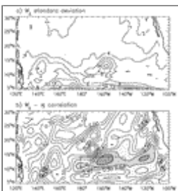
FIG. 9. (a) Standard deviation of the Ekman pumping anomalies. Units are 10^{-5} \text{ cm s}^{-1} . (b) Instantaneous correlation between Ekman pumping anomalies and 25.5 \sigma_\theta isopycnal depth anomalies. Note that the sign of the depth anomalies has been reversed, so that positive correlations correspond to negative W'_E and positive \eta' (deepening of the isopycnal), and vice versa. Contour interval is 0.1. Values larger than 0.6 are shaded
