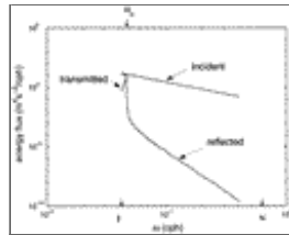
Fig. 1. Incident, reflected, and transmitted flux spectra as a function of modenumber and frequency for a half-cosine slope of depth ratio \delta = 4/32 and maximum slope h'_{\max} = 0.01\pi . Solid lines in the coordinate planes are the frequency and modenumber spectra.
