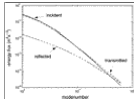
Fig. 2. Incident, reflected, and transmitted flux frequency spectra for the half-cosine slope of Fig. 1 🔍.
