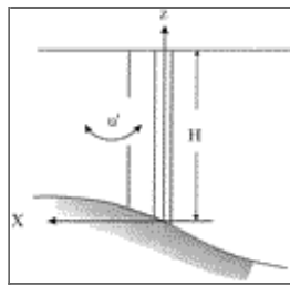
Fig. 1. The model configuration for the analytical model, in which a cross-shore tidal current interacts with a mean property field having vertical isolines.
