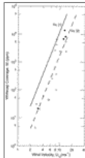
Fig. 2. Numbers of bubbles produced in fresh (+) and salt (●) waters. The results are reproduced from Loewen et al. (1996) .
