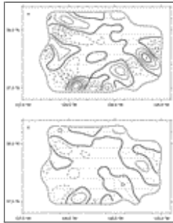
Fig. 4. At 100 m, (a) IG1 streamfunction \psi_1 scaled by f(\text{m}^2 \text{ s}^{-2}) computed from (13) and absolute dynamic height ( \text{m}^2 \text{ s}^{-2} ) (gray contours); and (b) IG1 velocity potential \chi_1 scaled by f(\text{m}^2 \text{ s}^{-2}) and divergent velocity vectors \mathbf{u}_{1D} computed from (10)
