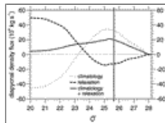
Fig. 10. Annual-mean water mass diagnostics evaluated over the whole basin for (a) the diffusive density flux D(\rho) ( 10^6 \text{ kg s}^{-1} ), (b) the diapycnal volume flux G(\rho) (Sv), and (c) the water mass formation rate M(\rho) = -\partial G/\partial \rho , ( \text{Sv}/\text{kg m}^{-3} ) all over the range 20 < \rho < 28 . For the density flux, the surface contribution D_{\text{surf}} is denoted by a thin dotted line, the mixing by a dashed line, the net contribution D_{\text{net}} from the sum of the surface forcing and mixing by a thin full line, and that consistent with the model truth by the thick solidline. In the plots of the diapycnal volume flux and formation rates, independent model truth is denoted by a thick full line. The gray bar at \sigma = 25.65 denotes the density of the lightest thermocline waters resolved by the model.
