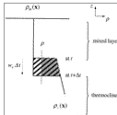
Fig. 6. The diffusive diapycnal flux D_{\text{diff}} acting in the interior of the ocean is split into components due to (a) lateral mixing in the mixed layer D_{\text{lat}} , (b) entrainment mixing at the base of the mixed layer D_{\text{ent}} , and (c) mixing within the thermocline proper D_{\text{thermo}} .
