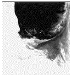
Fig. 2. NOAA infrared image. Grayscale from white (cold) to black (warm), with white clouds over land. Two Natal pulses are visible as cyclonic meanders in the relatively dark (warm) Agulhas Current between Durban and Port Elizabeth.
