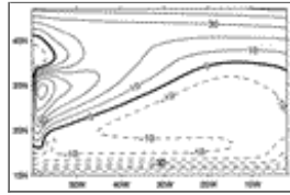
FIG. 2. Mean zonal wind stress W_z used in all the experiments (units: \text{N m}^{-2} )
