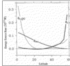
Fig. 1. Density distribution and potential energy sources. The upper panels show the density distribution, and the lower panels show the potential energy source due to mixing in the physical state (solid line) and in the reference state (dashed line).
