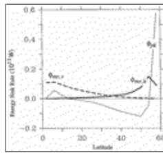
Fig. 3. APE sinks (integrated over each 4^\circ latitude band): \phi_{mn, v} is due to vertical mixing, \phi_{mr, h} is due to horizontal mixing, and \phi_{pk} is the rate that potential energy is converted to kinetic energy.
