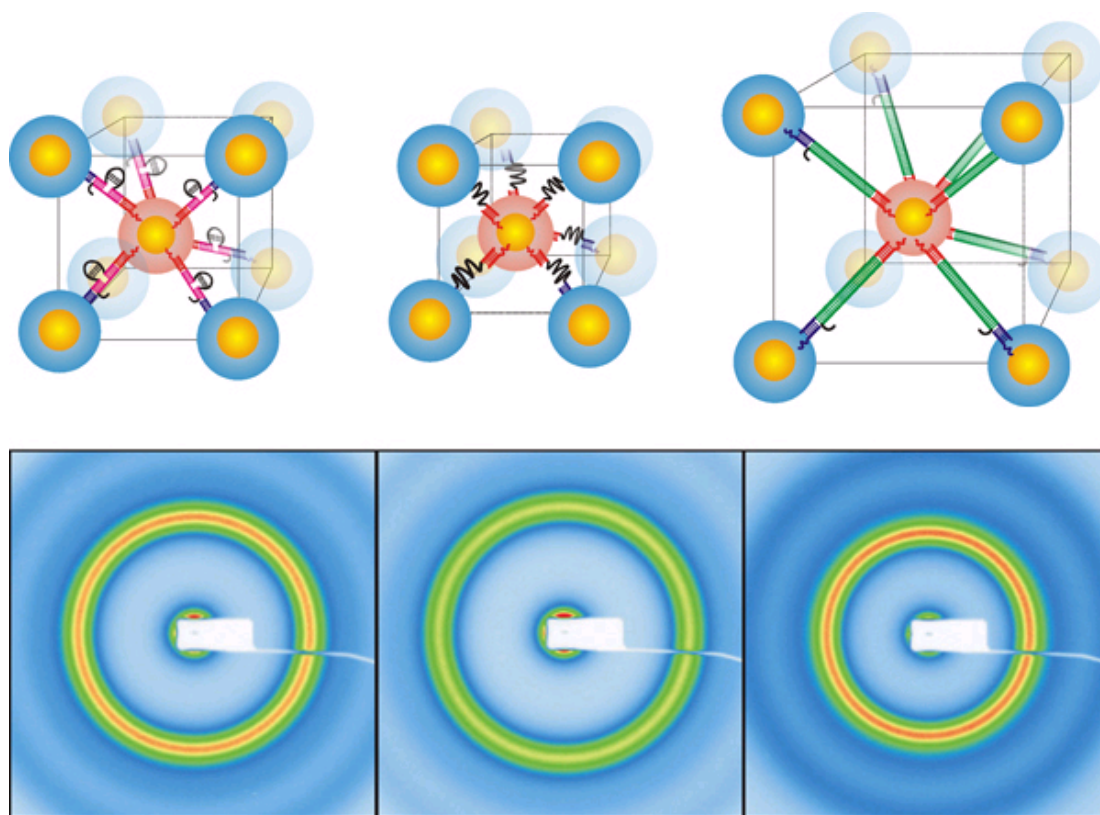
These illustrations show how a 3-D crystal made from nanoparticles changes between two distinct states via an intermediate structure (top row, middle) when looped (left) versus unlooped (right) double-stranded DNA chains are used to link the particles. The scientists were able to measure the distance between the particles in each structure by recording x-ray scattering patterns (bottom row). Switching from looped to unlooped DNA increased the interparticle distance by about 6 nanometers. + ENLARGE
