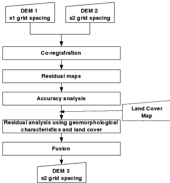
Figure 1: Workflow of the DEM fusion approach.
