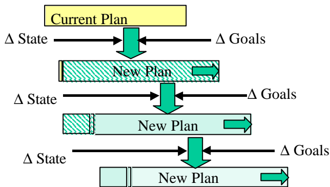
Figure 5. Continuous Planning Incremental Plan Extension
