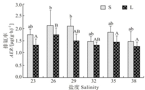
图4 不同盐度条件下红刺参排氨率 Fig.4 Ammonia-N excretion rate of red type A. japonicus at different salinities
