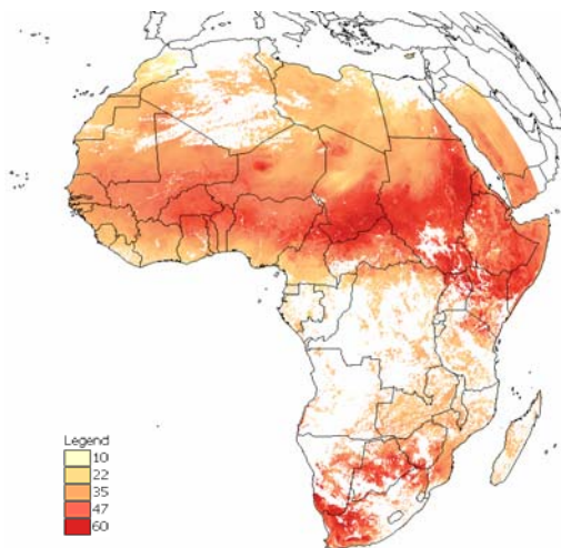
Figure 7: Land Surface Temperature
