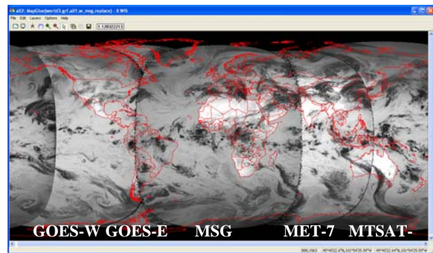
Figure 8: Foreign Satellite thermal infrared global composite
