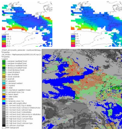
Figure 3. K-index, precipitable water and cloud analysis image
