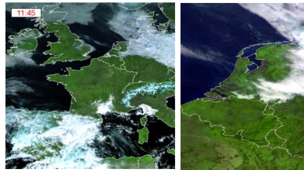
Figure 1. Near real-time Meteosat visualization
