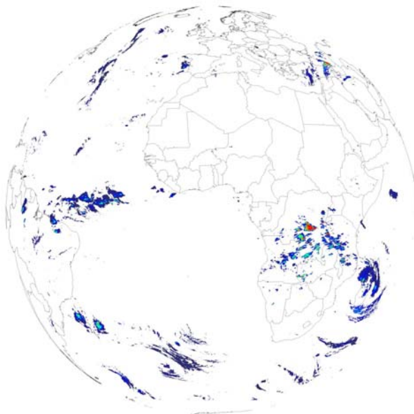
Figure 4. Multi Sensor Precipitation Estimate
