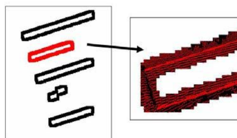
Figure 5. Dispersed points spread on the grid.
