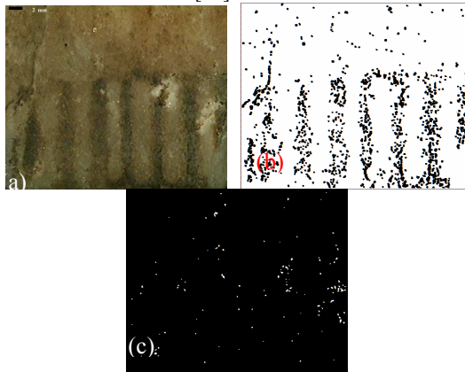
Figure 7: (a) Stone material (monitored by a reflectography system (vis)) demonstrating cleaned and un-cleaned stripes, (b) Black particles detected, (c) white particles detected.
