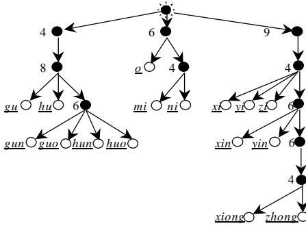
FIGURE 1. PART OF THE SYLLABLE-DIGIT TREE
