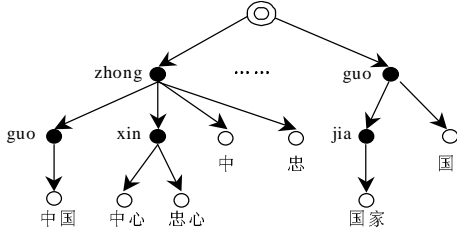
FIGURE 2. PART OF THE WORD SYLLABLE TREE
