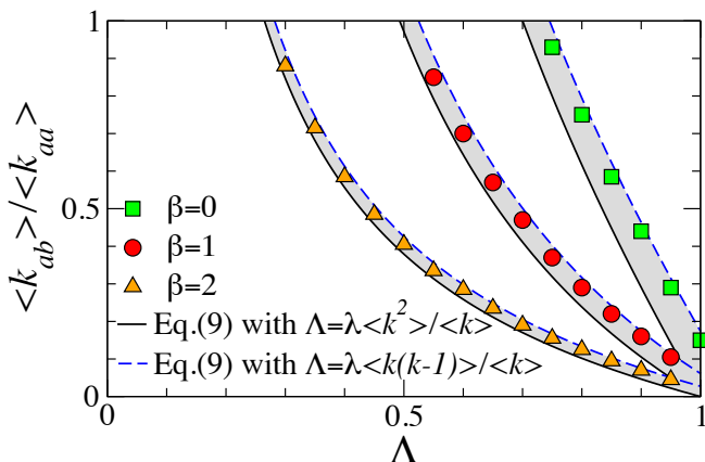
FIG. 3: Critical lines for \beta = 0, 1, 2 for the same networks as in Fig. 2. Dotted lines correspond to numerical simulations, black lines are the theoretical predictions according to Eq. (9), whereas blue dashed lines are obtained by rescaling the \Lambda axis as \Lambda \rightarrow \Lambda(1 - \langle k \rangle / \langle k^2 \rangle)^{-1} .
