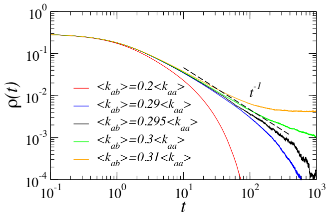
FIG. 2: Time evolution of the prevalence \rho(t) below and above the critical point for \Lambda = 0.8 for two identical networks interconnected with linear correlations, i. e. , \beta = 1 . Each network has an exponential degree distribution with \langle k \rangle = 10 and minimum degree 2. The size of each network is N = 10^6 and results are averaged over 100 different realizations of the process. Right at the critical point, the prevalence decays as \rho(t) \sim t^{-1} .
