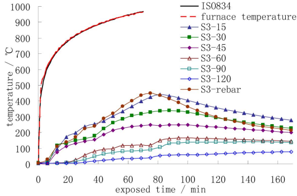
Fig. 6 Temperature histories of S3
