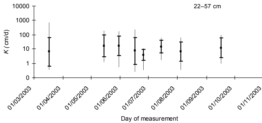
Figure 7. Temporal course and spatial variability of the K_{\text{labor}} values measured for the soil profile layer 22–57 cm on the samples taken during the year 2003 in Most pri Bratislave, expressed by the values of maximum, minimum, arithmetic mean, and the standard deviation from the mean (thin lines)
