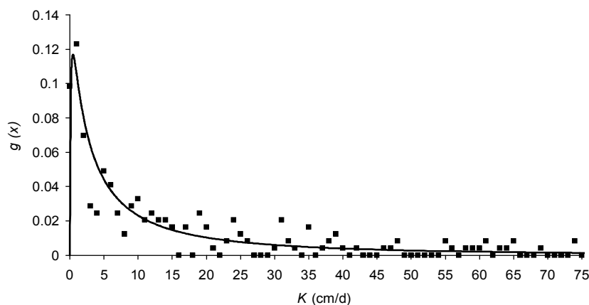
Figure 3. Empirical relative frequency and theoretical density of the log- normal distribution of the K_{\text{labor}} values, for all measurements performed on the samples taken during the period 17. 3.–15. 10. 2003 in the soil horizon 0–120 cm, in the locality Most pri Bratislave
