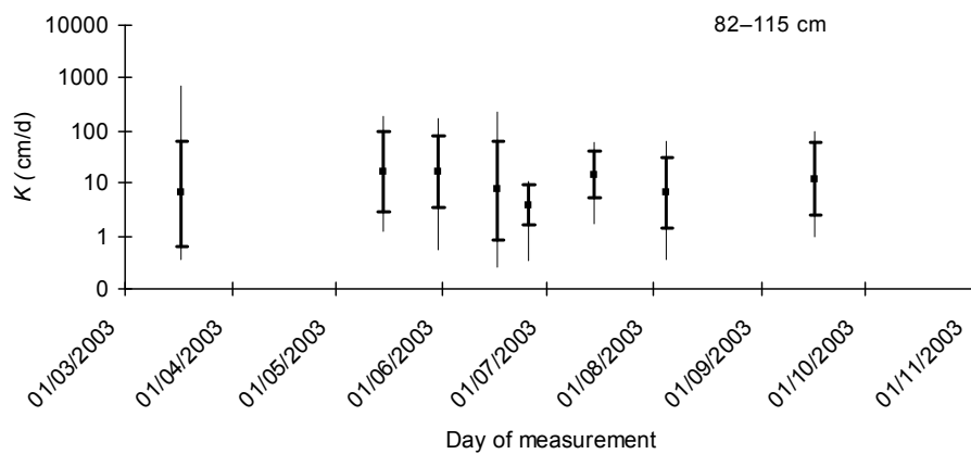
Figure 9. Temporal course and areal variability of the K_{\text{labor}} values measured for the soil profile layer 82–115 cm on the samples taken during the year 2003 in Most pri Bratislave, expressed by the values of maximum, minimum, arithmetic mean, and the standard deviation from the mean (thin lines)
