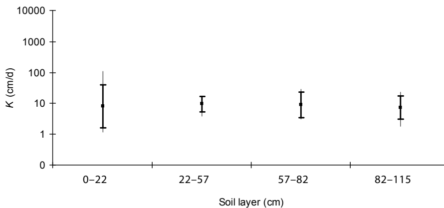
Figure 11. Temporal variability of the K_{\text{labor}} mean values in the 2003 vegetation period on the Most pri Bratislave locality; for several layers (0–22; 22–57; 57–82, and 82–115 cm) of the soil profile, expressed by the values of maximum, minimum, arithmetic mean, and the standard deviation from the mean (thin lines)
