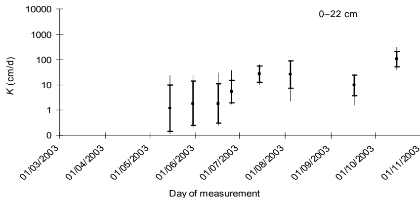
Figure 6. Temporal course and areal variability of the K_{\text{labor}} values measured for the soil profile layer 0–22 cm on the samples taken during the year 2003 in Most pri Bratislave, expressed by the values of maximum, minimum, arithmetic mean, and the standard deviation from the mean
