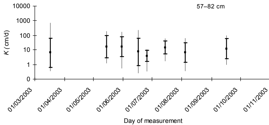
Figure 8. Temporal course and areal variability of the K_{\text{labor}} values measured for the soil profile layer 57–82 cm on the samples taken during the year 2003 in Most pri Bratislave, expressed by the values of maximum, minimum, arithmetic mean, and the standard deviation from the mean (thin lines)
