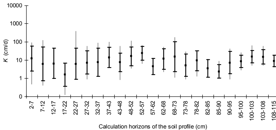
Figure 10. Temporal variability of the K_{\text{labor}} values determined in the samples taken on the sampling days of the 2003 vegetation period on the Most pri Bratislave locality, in several calculation horizons of the soil profile, expressed by the values of maximum, minimum, arithmetic mean, and the standard deviation from the mean (thin lines)
