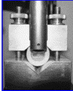
FIGURE 3. Application of force on composite block by the stub-shaped apparatus
