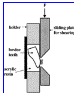
FIGURE 1. Schematic drawing of shear bond strength measurements
