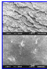
FIGURE 8. Scanning electron micrograph of typical fracture surfaces of the polycarbonate composite resin after shear bond test (above: resin cohesive fracture; below: resin-cement interface failure)
