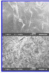
FIGURE 9. Scanning electron micrographs of typical polycarbonate composite resin bracket surfaces with (above) and without (below) 50% TEGDMA/MMA primer
