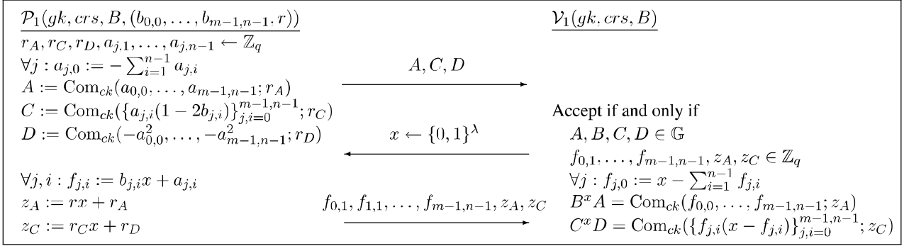
Fig. 4. \Sigma -protocol for relation \mathcal{R}_1 .
