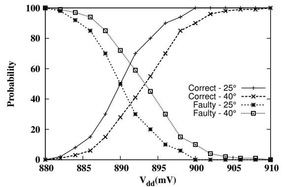
Fig. 2. Percentage of correct and faulty computations as a function of V_{dd} and temperature
