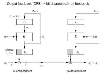
Figure 4: OFB Operation Mode of block ciphers
