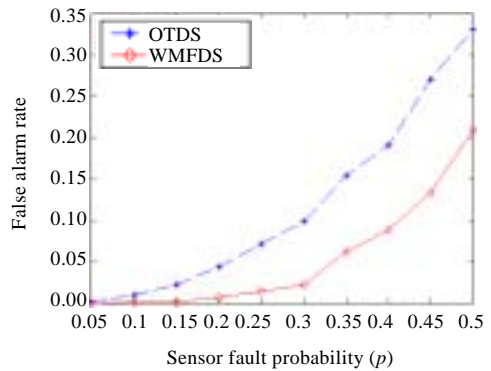
Fig.5 False alarm rate of binary decisions
