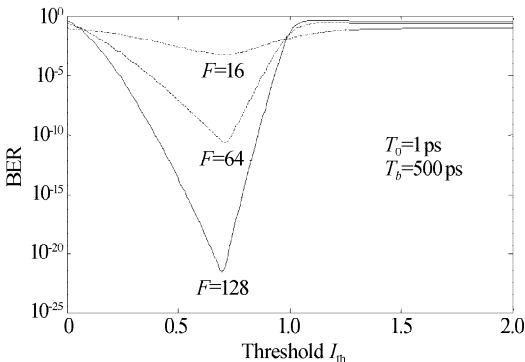
Fig. 2 The BER versus threshold for different F
