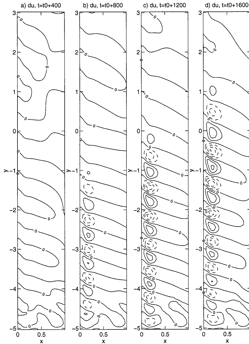
FIG. 10. Zonal velocity anomalies for the basic state described in Fig. 9 at intervals of \Delta t = 400 showing the development of the eddy field after the time t_0 = 1000 when the Reynolds number of the system was adjusted from 24 to 28.
