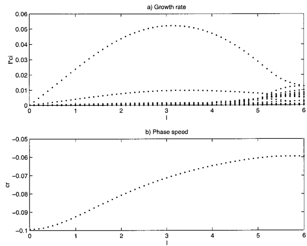
FIG. 3. (a) Growth rates as a function of meridional wavenumber for the velocity profile in Fig. 2 in the inviscid shallow-water system. Decaying modes (not shown) are complex conjugate solutions. (b) Phase speeds for the fastest growing modes in (a).
