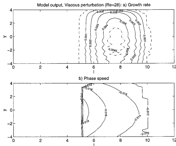
FIG. 9. As functions of meridional wavenumber and latitude, (a) growth rates and (b) phase speeds of the most unstable modes for the basic state (not shown) with \delta_M = 0.05 , using a viscosity of A_H = 1.071 \times 10^{-4} ( Re = 28 for the perturbations). The dashed contour corresponds to a value of \omega_i = 10^{-4} and divides the domain into regions of growth and regions of stability.
