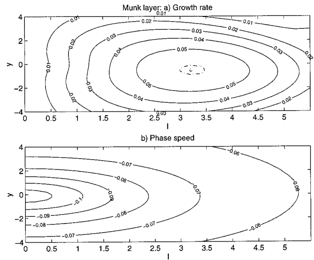
FIG. 5. As functions of meridional wavenumber and latitude, the (a) growth rate and (b) phase speed of the fastest growing mode for the Munk boundary layer in Fig. 2. The dot-dashed curves in (a) mark \omega_i = 0.058 and 0.0584 .
