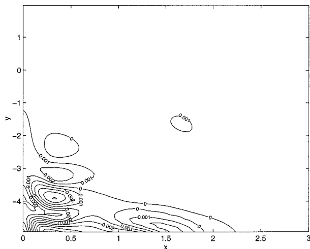
FIG. 8. The height field anomaly after instability begins. The difference in height fields between steady solution at Re = 31.25 to Re = 32.25 after 300 time units.
