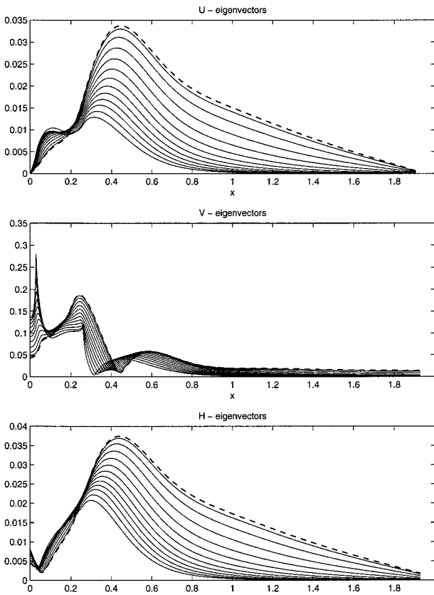
FIG. 4. Eigenfunction amplitudes of the most unstable modes in Fig. 3 at intervals of l = 0.5 : (a) U , (b) V , and (c) H . The dashed curve corresponds to l = 0.01 .
