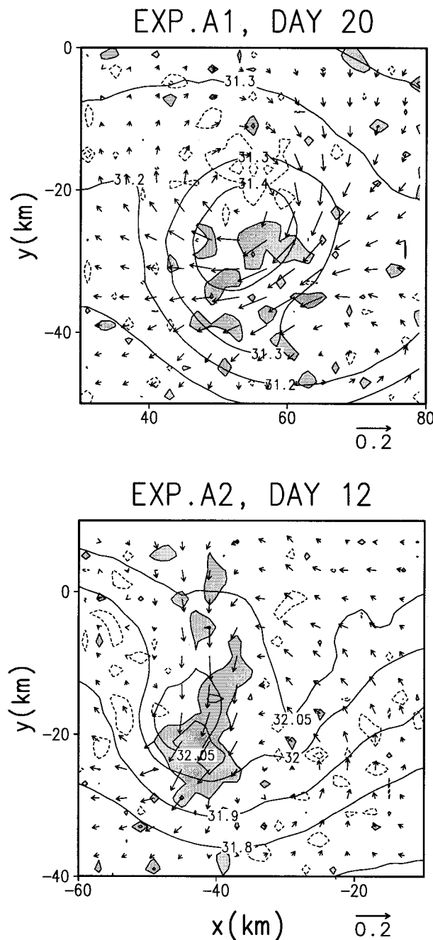
FIG. 8. Vertical velocity at z = -200 m superimposed on salinity (psu) and horizontal flow fields at 100 m for anticyclones A1 at day 20 (top) and A2 at day 12 (bottom). Solid contour lines show w = -0.01 and -0.02 \text{cm s}^{-1} , and dashed contour lines indicate w = 0.01 and 0.02 \text{cm s}^{-1} . Shading indicates downwelling speeds greater than 0.01 \text{cm s}^{-1} . Calibration arrow for horizontal flow is 0.2 \text{m s}^{-1} .
