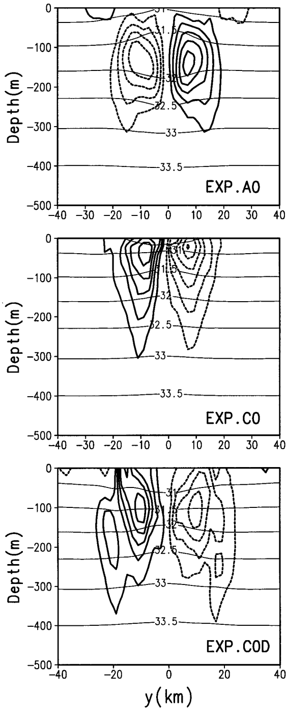
FIG. 4. Salinity in psu (thin lines) and azimuthal velocity (thick lines) in the y - z plane at day 20 in experiments A0 (top), C0 (middle), and C0D (bottom). Dashed and solid isotachs are into and out of the paper, respectively, with the outermost isotachs at \pm 2 \text{ cm s}^{-1} and a contour interval of 2 \text{ cm s}^{-1} .
