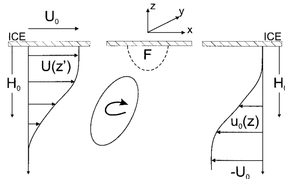
FIG. 2. Side view of an eddy in a coordinate system moving with the ice cover at speed U_0 . The current profiles in the ice- and land-based coordinate systems are shown on the right and left, respectively. The eddy is generated beneath the source F . When being swept backward, an anticyclone (cyclone) tilts and moves laterally toward the -y ( +y ) direction in the Northern Hemisphere with the lower part of the eddy leading. In this illustration the submerged eddy is anticyclonic; the lower part of the eddy should be displaced out of the paper.
