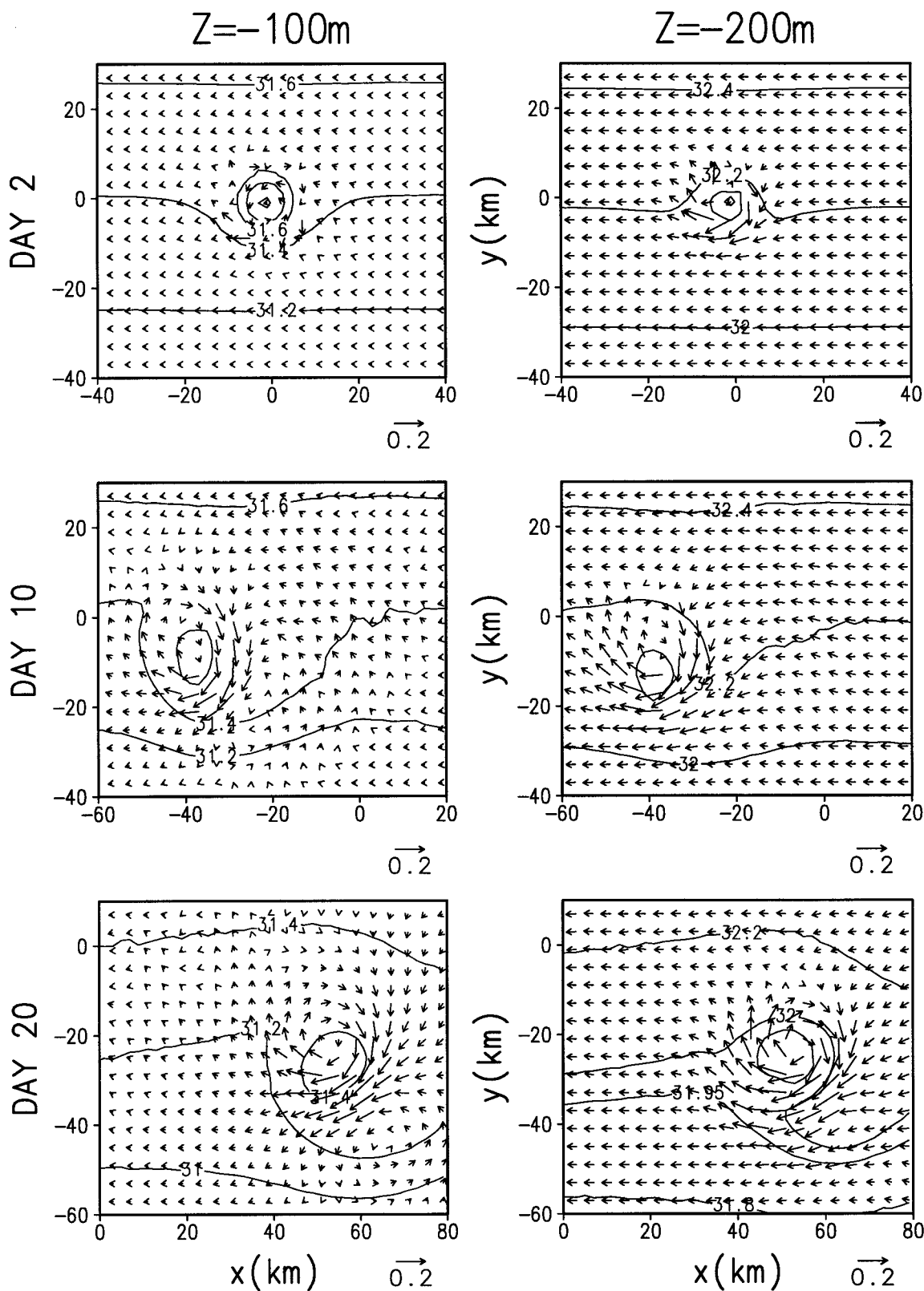
FIG. 6. Flow and salinity (psu) fields near anticyclone A1 at z = -100 m (left) and -200 m (right) at day 2 (top), day 10 (middle), and day 20 (bottom) in the frame moving with the ice cover. The calibration arrow for velocity is 0.2 \text{ m s}^{-1} .
