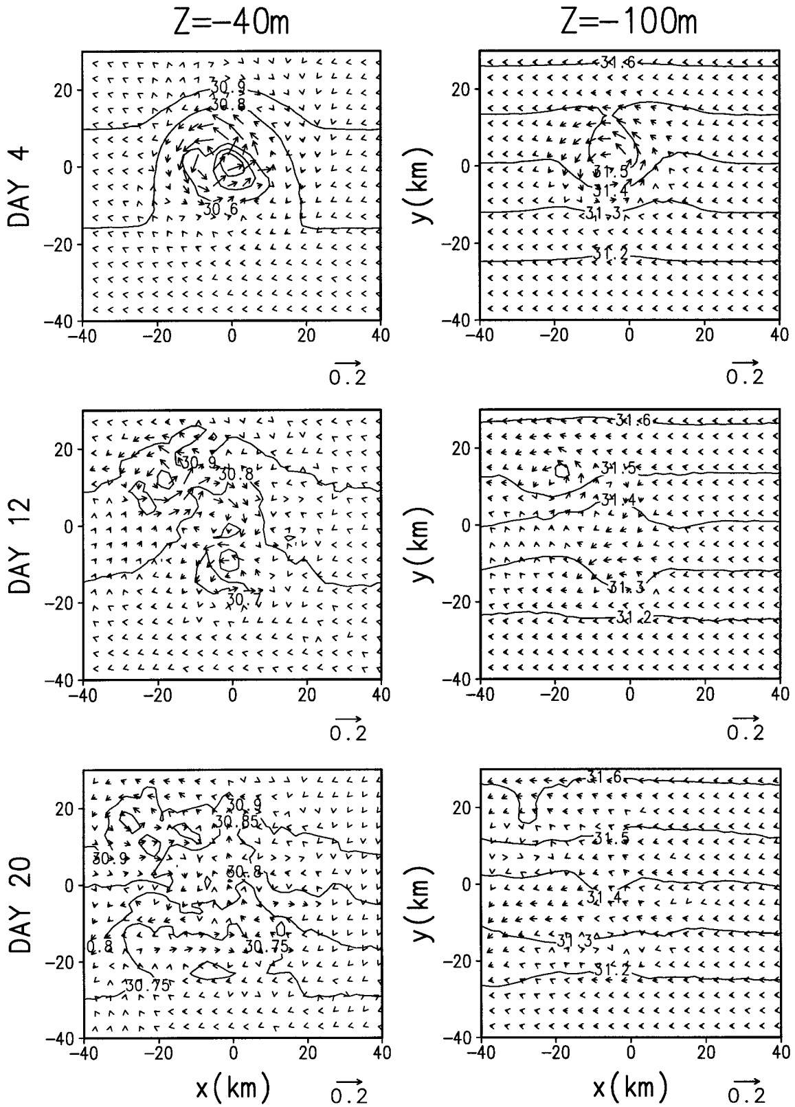
FIG. 9. Flow and salinity (psu) fields near cyclone C1 at depths of 40 m (left) and 100 m (right) at day 4 (top), day 12 (middle), and day 20 (bottom). Calibration arrow is 0.2 \text{ m s}^{-1} .
