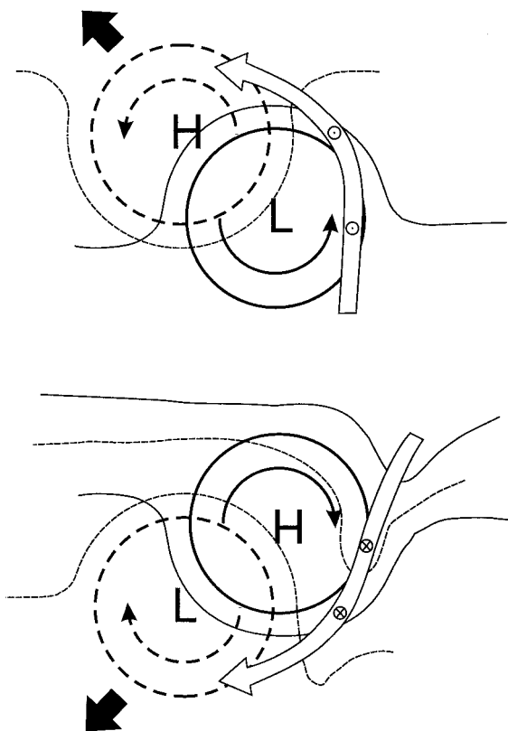
FIG. 13. Schematic plane views of circulations near a tilted cyclone (top) and anticyclone (bottom) in the westward ambient current shown in Fig. 2 from an observer moving with the ice cover. Solid and dashed lines indicate features associated with the upper and lower halves of an eddy, respectively. Density surpluses and deficits are marked by H and L. Large open arrows with associated upwelling ( \odot ) and downwelling ( \otimes ) indicate the jet trailing an eddy. Large solid arrows indicate directions of eddy drift relative to ice.
