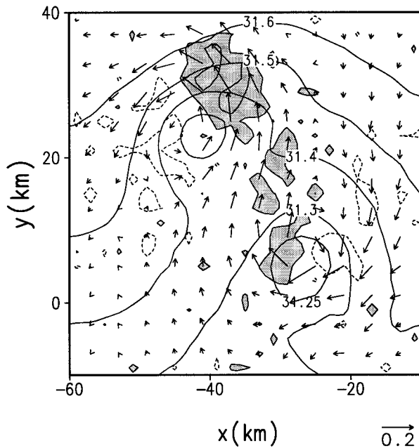
FIG. 11. Vertical velocity at z = -200 m superimposed on salinity (psu) and horizontal flow fields at 100 m for cyclone C3 at day 12. Contour lines, shading and calibration arrow length are the same as those in Fig. 8.
