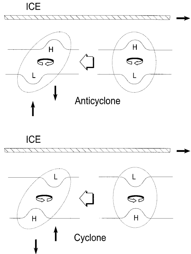
FIG. 12. Schematic side views of eddies experiencing a sudden, large tilt. Vertical velocities are triggered to disperse an anticyclone (top) and a cyclone (bottom). Symbols H and L denote density surpluses and deficits relative to surrounding waters, respectively.
