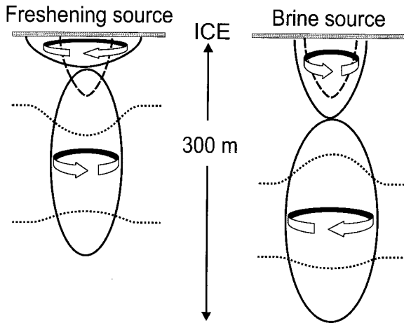
FIG. 1. A schematic sectional view showing how a freshening or a brine source in an initially quiescent ocean generates vertically stacked pairs of counterrotating eddies. Dashed contours beneath the ice cover indicate a region where a freshening or a brine source is applied. Dotted contours indicate isohalines associated with eddy pairs. Top eddies are damped by surface friction in time.
