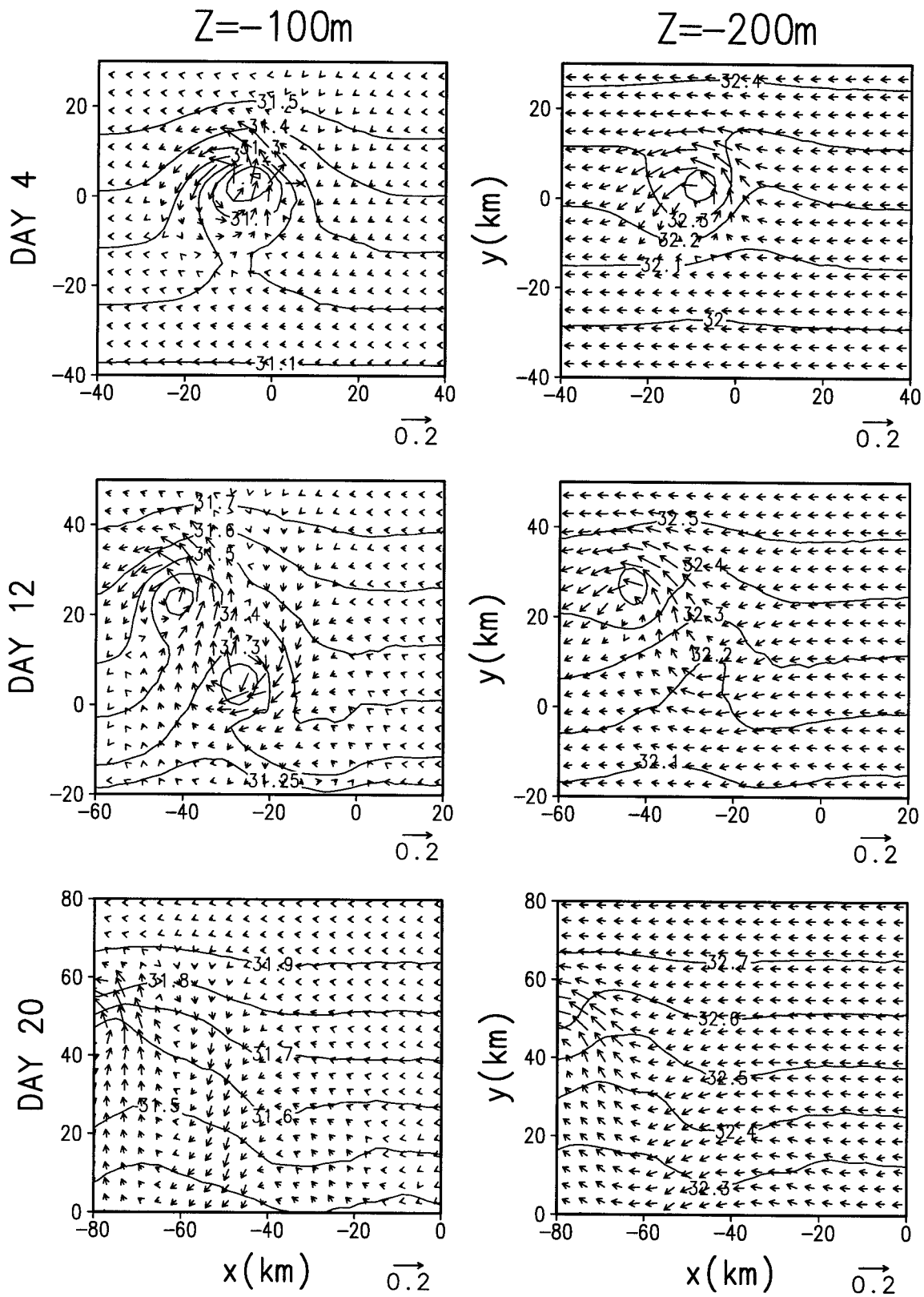
FIG. 10. Same as Fig. 9 but for cyclone C3 at depths of 100 m (left) and 200 m (right). The cyclone has dispersed at day 20.
