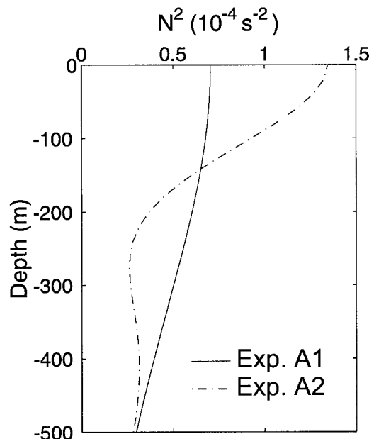
FIG. 3. Profiles of N^2 at the center latitude of the basin for experiments A1 and A2. Since N^2 varies linearly with y at a fixed depth, difference between the two profiles remains at all other latitudes. Specifically, stratification below 140-m depth is always stronger in A1 than in A2.
