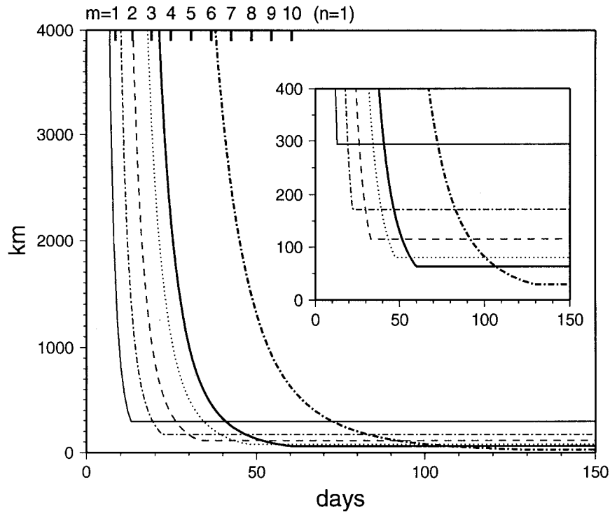
FIG. 8. Width of the fluctuating western boundary layer vs the forcing period according to (17) for A_H = 500\,000\text{ m}^2\text{ s}^{-1} (thin solid line), A_H = 100\,000\text{ m}^2\text{ s}^{-1} (thin dashed-dotted line), A_H = 30\,000\text{ m}^2\text{ s}^{-1} (thin dashed line), A_H = 10\,000\text{ m}^2\text{ s}^{-1} (thin dotted line), A_H = 5\,000\text{ m}^2\text{ s}^{-1} (thick solid line), A_H = 500\text{ m}^2\text{ s}^{-1} (thick dashed-dotted line).
