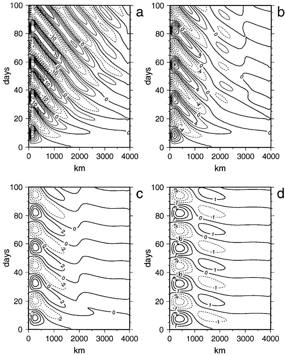
FIG. 1. Hovmöller diagrams of the meridional velocity v (in \text{mm s}^{-1} ) solution of (2) forced by (1) with \omega = \omega_{41} ( T = 24.79 days) along a zonal section equidistant from the northern and southern boundaries with (a) A_H = 10\,000 \text{ m}^2 \text{ s}^{-1} , (b) A_H = 30\,000 \text{ m}^2 \text{ s}^{-1} , (c) A_H = 100\,000 \text{ m}^2 \text{ s}^{-1} , (d) A_H = 500\,000 \text{ m}^2 \text{ s}^{-1} .
