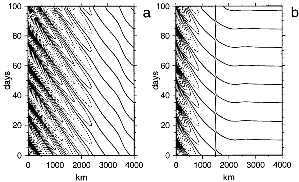
FIG. 3. Hovmöller diagrams of the meridional velocity v given by expression (9) with (10) and \omega = \omega_{41} ( T = 24.78 days) along a zonal section equidistant from the northern and southern boundaries with (a) A_H = 10\,000\text{ m}^2\text{ s}^{-1} (cf. Fig. 1a), (b) A_H = 30\,000\text{ m}^2\text{ s}^{-1} (cf. Fig. 1b).
