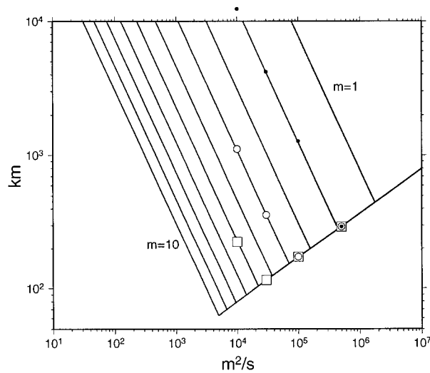
FIG. 5. Width of the fluctuating western boundary layer l vs the horizontal eddy viscosity coefficient A_H according to (16) for the first 10 zonal eigenperiods given in Table 1. The white circles denote the experiments of Fig. 1, the dots those of Fig. 6, and the squares those of Fig. 7.
