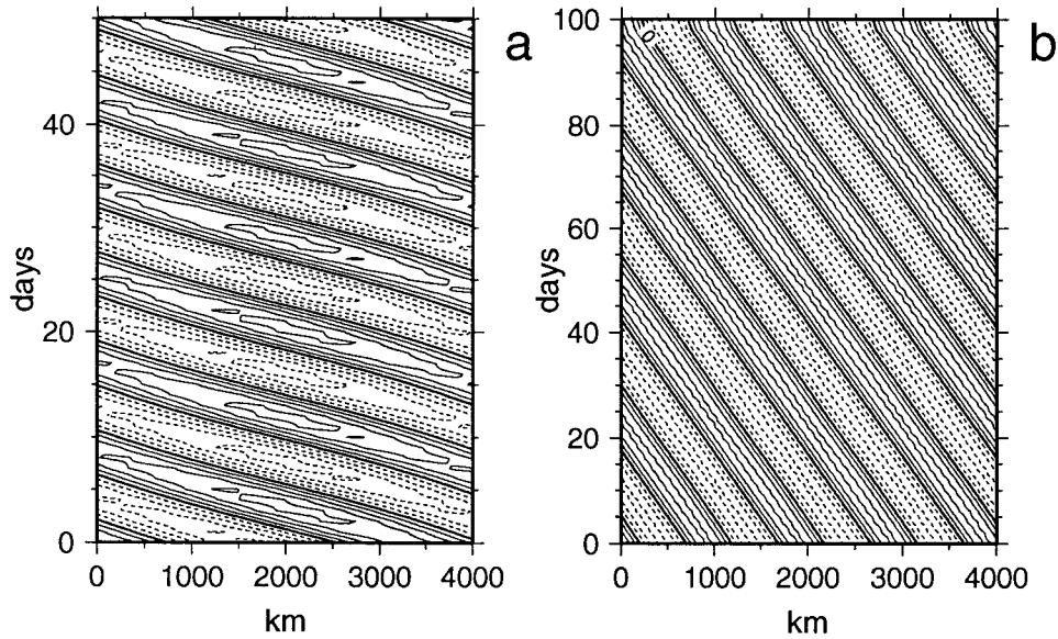
FIG. 2. Hovmöller diagrams of the meridional velocity v given by the analytical inviscid nondivergent normal modes (1, 1) (a) and (4, 1) (b) given by (5) or (6) with (7) along a zonal section equidistant from the northern and southern boundaries.
