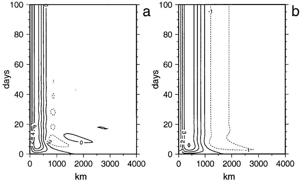
FIG. 4. Hovmöller diagrams of the meridional velocity v (in \text{mm s}^{-1} ) solution of (2) forced by a wind stress curl constant both in space and time along a zonal section equidistant from the northern and southern boundaries with (a) A_H = 100\,000 \text{ m}^2 \text{ s}^{-1} (cf. Fig. 1c), (b) A_H = 500\,000 \text{ m}^2 \text{ s}^{-1} (cf. Fig. 1d).
