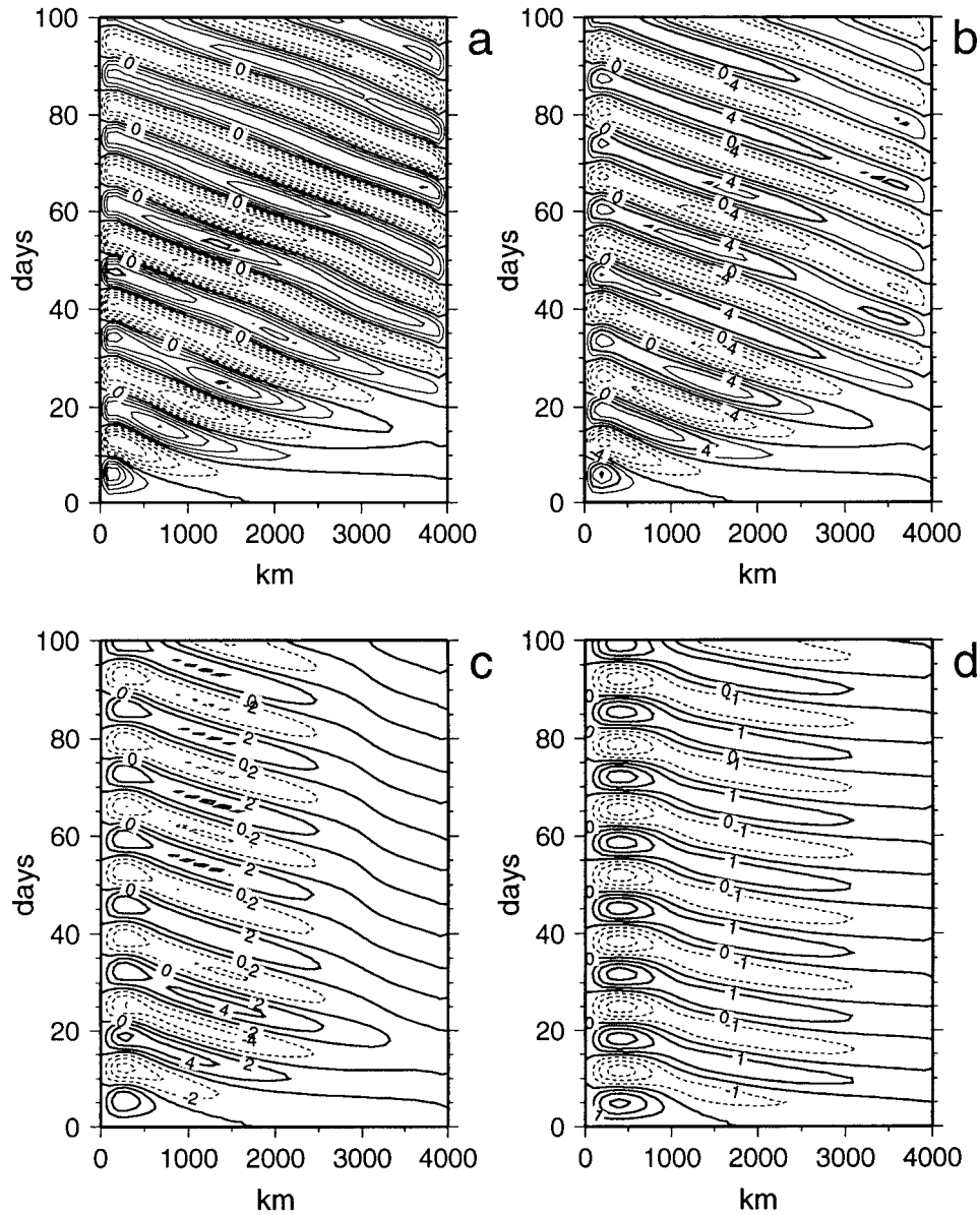
FIG. 6. Hovmöller diagrams of the meridional velocity v (in \text{mm s}^{-1} ) solution of (2) forced by (1) with \omega = \omega_{21} ( T = 13.44 days) along a zonal section equidistant from the northern and southern boundaries with (a) A_H = 10\,000 \text{ m}^2 \text{ s}^{-1} , (b) A_H = 30\,000 \text{ m}^2 \text{ s}^{-1} (c) A_H = 100\,000 \text{ m}^2 \text{ s}^{-1} , (d) A_H = 500\,000 \text{ m}^2 \text{ s}^{-1} .
