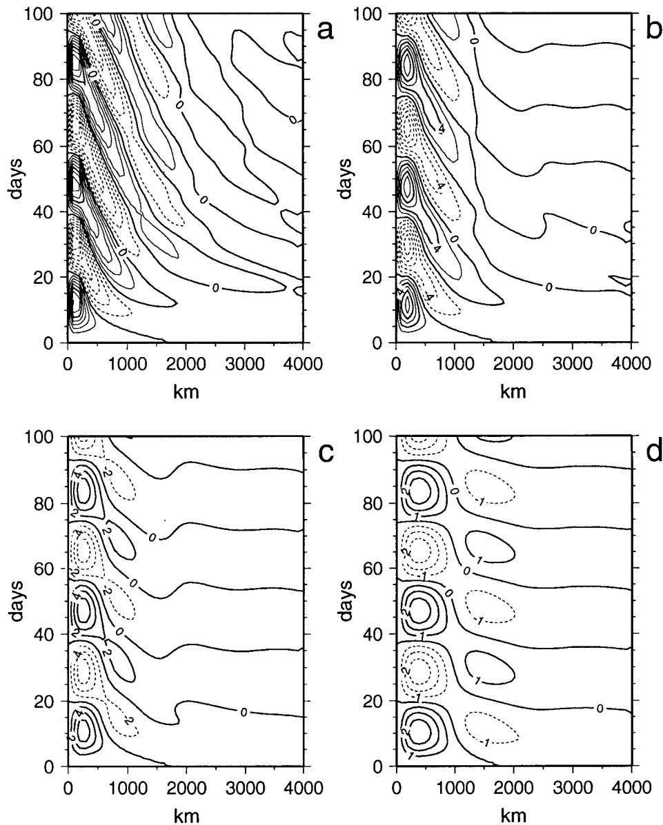
FIG. 7. Hovmöller diagrams of the meridional velocity v (in \text{mm s}^{-1} ) solution of (2) forced by (1) with \omega = \omega_{61} ( T = 36.57 days) along a zonal section equidistant from the northern and southern boundaries with (a) A_H = 10\,000 \text{ m}^2 \text{ s}^{-1} , (b) A_H = 30\,000 \text{ m}^2 \text{ s}^{-1} , (c) A_H = 100\,000 \text{ m}^2 \text{ s}^{-1} , (d) A_H = 500\,000 \text{ m}^2 \text{ s}^{-1} .
