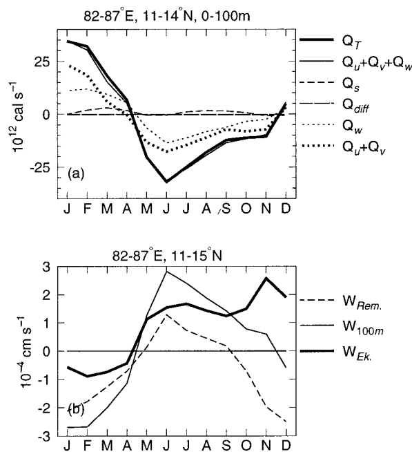
FIG. 12. As in Fig. 8 but for the Bay of Bengal dome, for the region shown by box B in Fig. 1.
