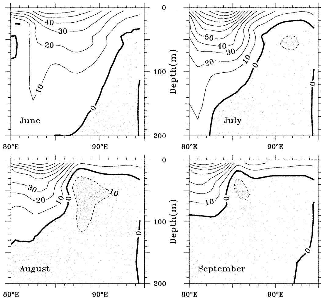
FIG. 17. Vertical section of zonal velocity along 5^{\circ}\text{N} , during the SWM. Contour interval is 10\text{ cm s}^{-1} . Thick contour represents zero. Westward flow is shaded as well as shown by dashed contours. Note the westward propagation of westward flow and the consequent reduction in thickness of the layer with eastward flow.
