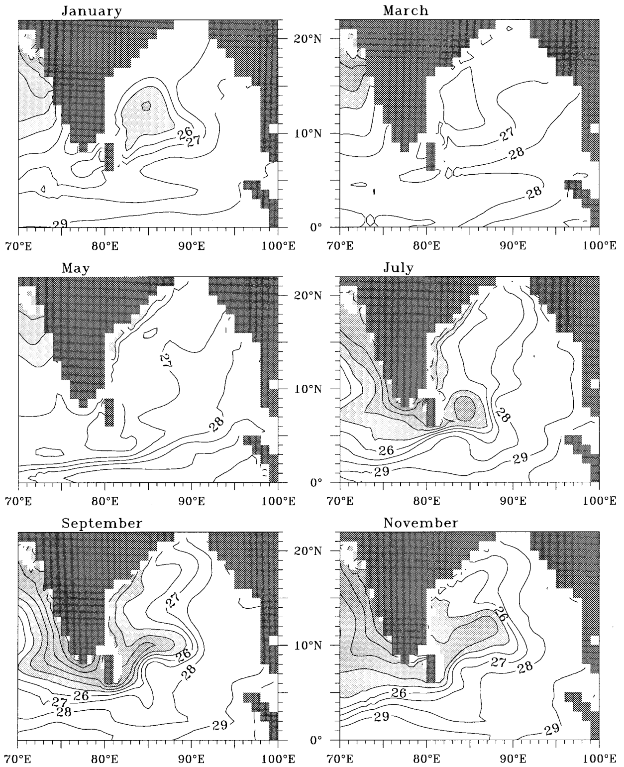
FIG. 5. Bimonthly maps of temperature from the model at a depth of 35 m. Contour interval is 1°C. Regions with temperature less than 25°C are shaded.
