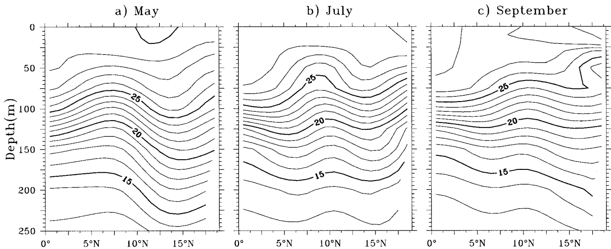
FIG. 2. Vertical section of climatological temperature (Levitus and Boyer 1994) along 85°E for the months of (a) May, (b) July, and (c) September. Contour interval is 1°C. Every fifth contour is marked by a thick line.
