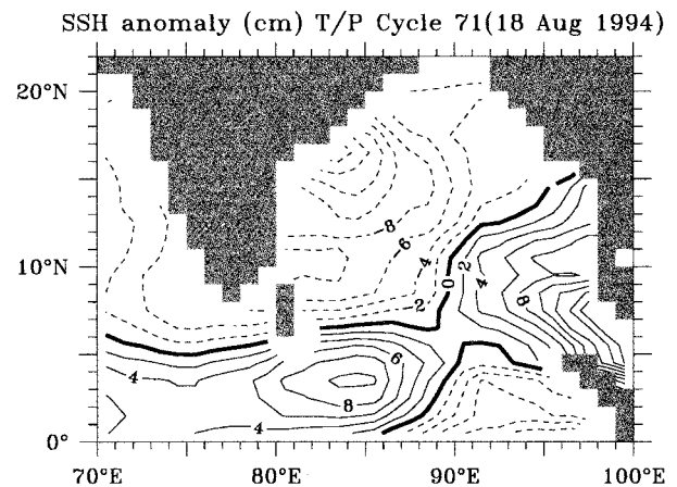
FIG. 15. Sea surface height (SSH) anomaly from TOPEX/Poseidon altimeter. The anomaly is defined as the difference from the mean SSH for the period November 1992–November 1996 (Tapley et al. 1994). Contour interval is 2 cm and negative anomalies are shown by dashed contours.
