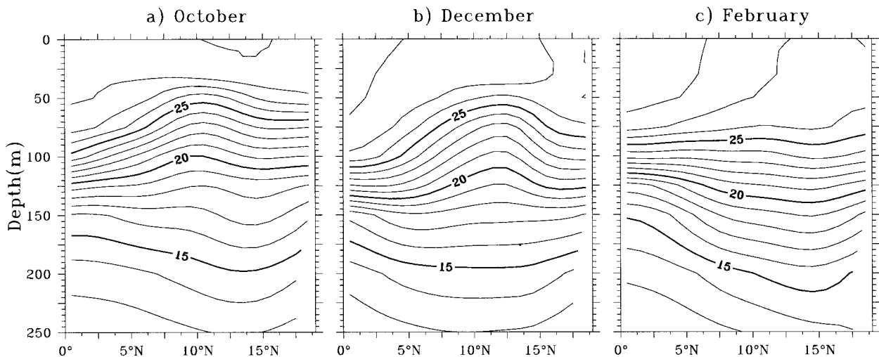
FIG. 3. Vertical section of climatological temperature (Levitus and Boyer 1994) along 85°E for the months of (a) October, (b) December, and (c) February. Contour interval is 1°C. Every fifth contour is marked by a thick line.
