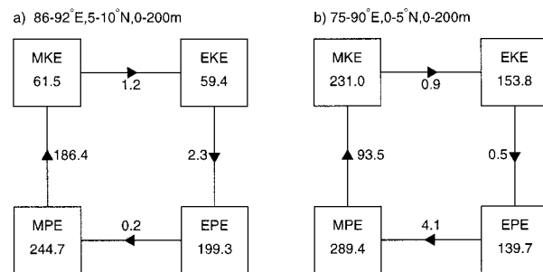
FIG. 13. Values of the energy components ( \text{cm}^2 \text{s}^{-2} ) and interaction terms ( 10^{-5} \text{cm}^2 \text{s}^{-3} ) for (a) the IG eddy east of the SLD and (b) for the anticyclonic vortex south of Sri Lanka. All terms calculated for the boxes are shown above the figures using the formulas given by Boning and Budich (1992). See text for acronyms.
