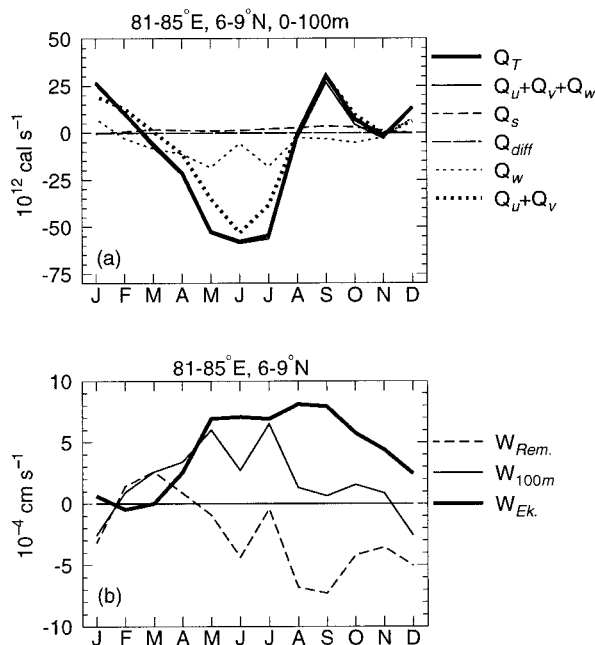
FIG. 8. (a) Heat balance analysis for the Sri Lanka dome. The dimensions of the box chosen (box A in Fig. 1) are shown at the top of the figure. The rate of change of heat storage ( Q_T ) is given by Q_T = Q_u + Q_v + Q_w + Q_s + Q_{diff} , where Q_u , Q_v , and Q_w are net zonal, meridional, and vertical fluxes; Q_s is the heat flux from the atmosphere; and Q_{diff} is the contribution from diffusive processes. (b) Vertical velocity at 107 m from the model (thin continuous line), Ekman pumping velocity (thick line), and the upwelling due to remote effects (dashed line). Remote upwelling is calculated as the difference between the model vertical velocity and Ekman pumping. All values are averaged over the horizontal region shown above the figure.
