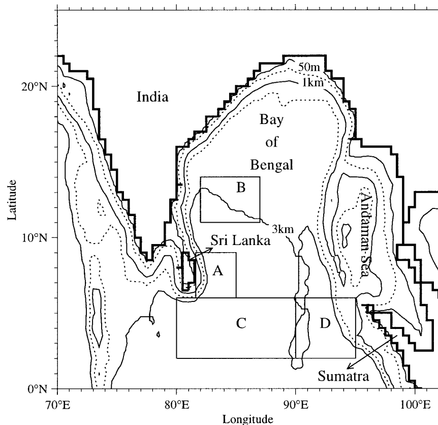
FIG. 1. Geometry of the coastline and bottom topography of the study area in the model. Thick line represents the land boundary in the model. Contours are isobaths. Dashed contours are for 200 m and 2 km. Boxes A, B, C, and D have reference to Figs. 8, 12, and 18.
