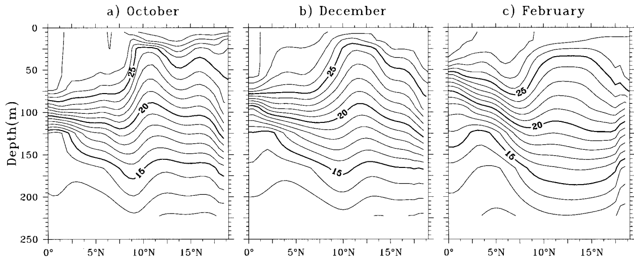
FIG. 11. Vertical section of temperature from the model, along 85°E for the months of (a) October, (b) December, and (c) February. Contour interval is 1°C. Every fifth contour is marked by a thick line.
