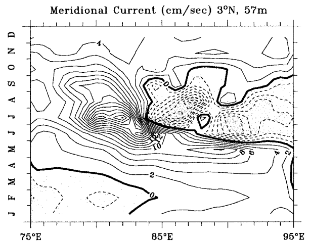
FIG. 16. Time–longitude section of meridional velocity from the model, at a depth of 57 m along 3^{\circ} N. Contour interval is 2 \text{ cm s}^{-1} . Regions with southward flow are shaded as well as shown by dashed contours.
