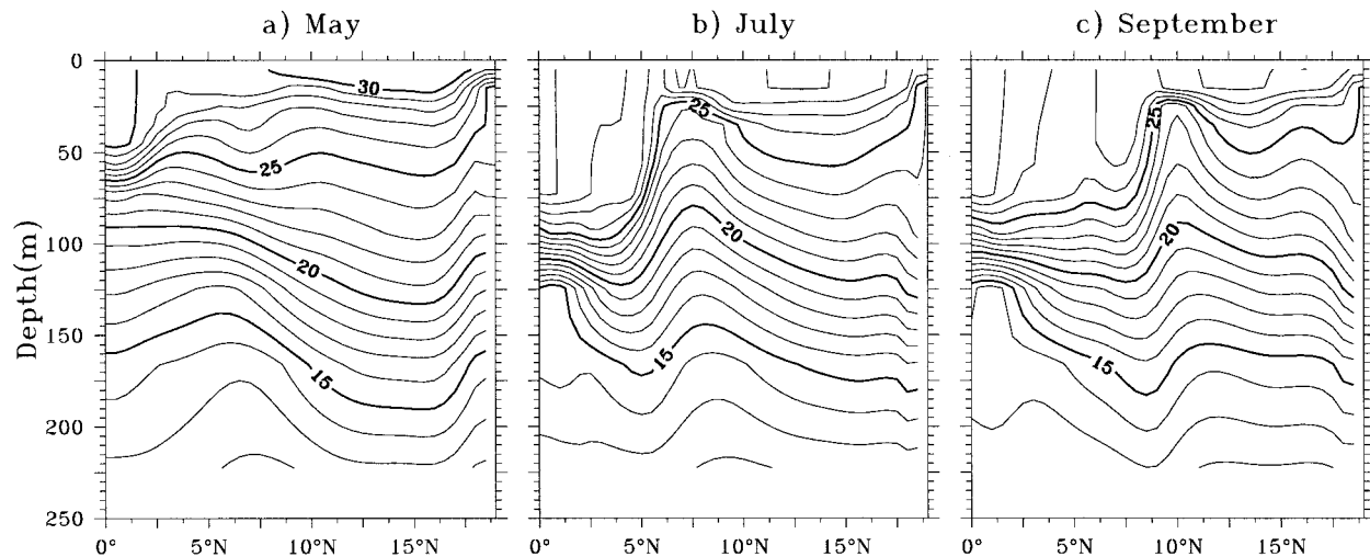
FIG. 6. Vertical section of temperature from the model, along 85°E for the months of (a) May, (b) July, and (c) September. Contour interval is 1°C. Every fifth contour is marked by a thick line.
