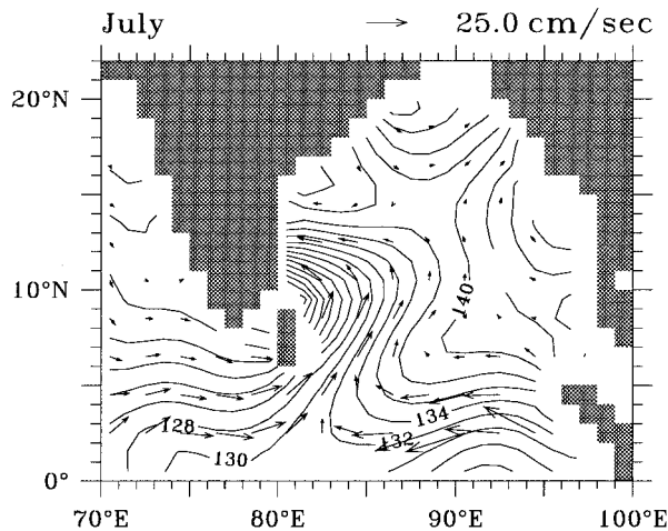
FIG. 14. As in Fig. 10 but for the month of July.
