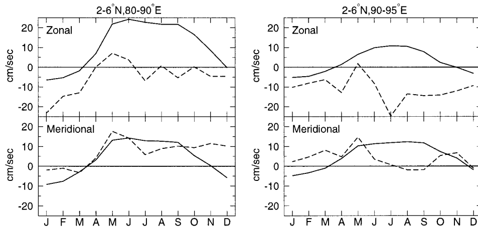
FIG. 18. Ekman (full line) and geostrophic (dashed) components of surface flow. Ekman components are calculated from the Hellerman and Rosenstein (1983) wind stress values using the formula used by Hastenrath and Greischar (1991). Geostrophic currents are calculated from dynamic heights (with reference to 500 m) based on climatological temperature (Levitus and Boyer 1994) and salinity (Levitus et al. 1994). Average values for the box C (Fig. 1) are shown in the left panel and that for box D (Fig. 1) are shown in the right panel.
