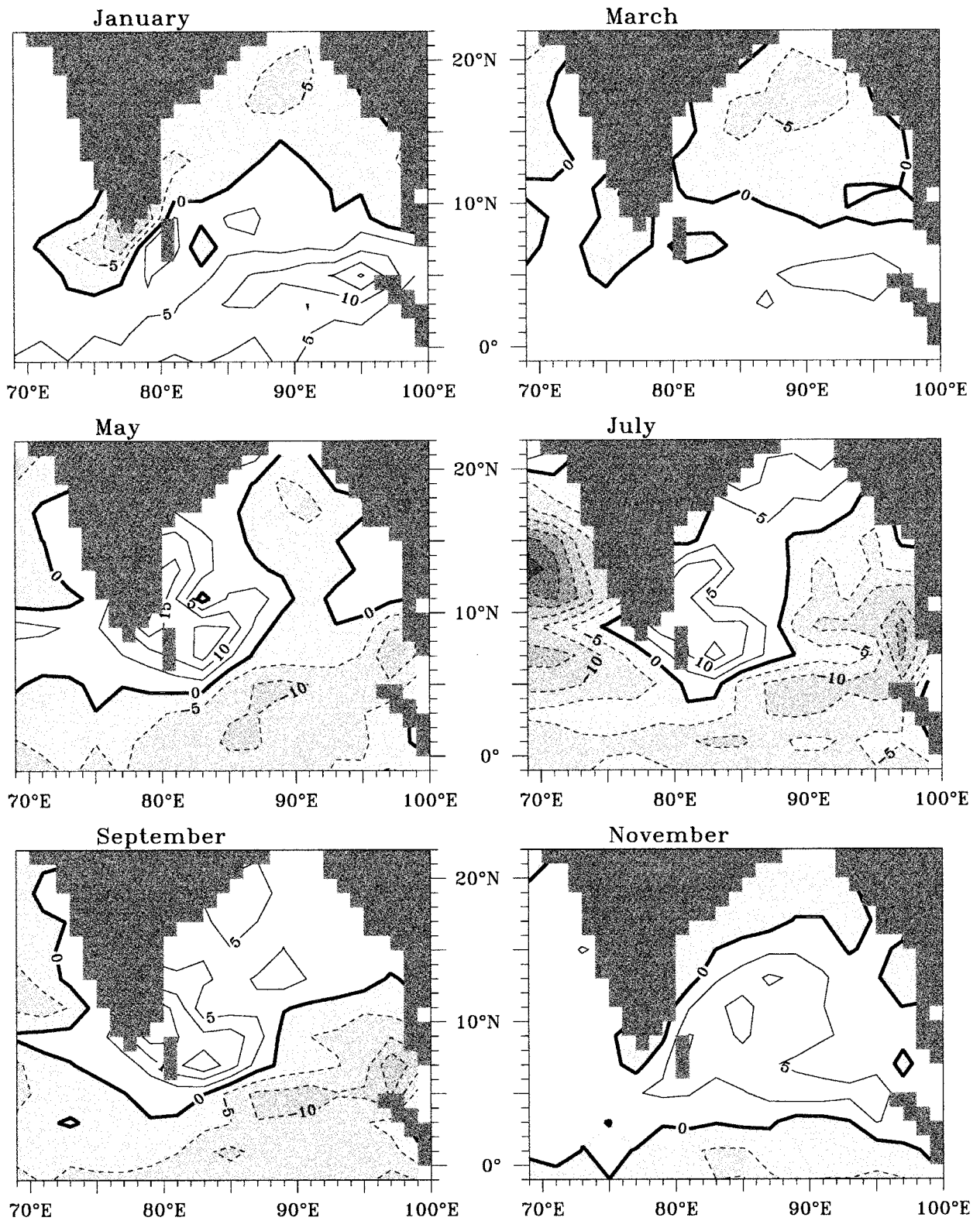
FIG. 7. Bimonthly maps of curl of the wind stress (Hellerman and Rosenstein 1983). Contour interval is 5 \times 10^{-9} \text{ dyn cm}^{-3} . Negative values are shaded. Note the strong cyclonic (anticlockwise) curl east of Sri Lanka and the strong anticyclonic (clockwise) curl near the eastern boundary during the southwest monsoon.
