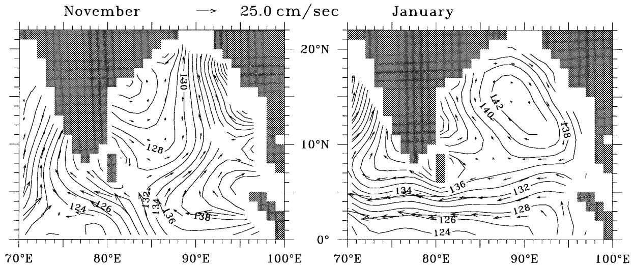
FIG. 10. Dynamic topography of the sea surface with reference to 500 m calculated from the climatological (Levitus and Boyer 1994; Levitus et al. 1994) data for the months of November (left panel) and January (right panel). Contour interval is 2 dyn cm. Arrows represent geostrophic currents.
