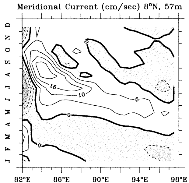
FIG. 9. Time-longitude section of meridional velocity from the model, at a depth of 57 m along 8°N. Contour interval is 5 cm s -1 . Regions with southward flow is shaded as well as shown by dashed contours. A Rossby wave signal radiating from the eastern boundary during April-June hits the east coast of Sri Lanka during September.
