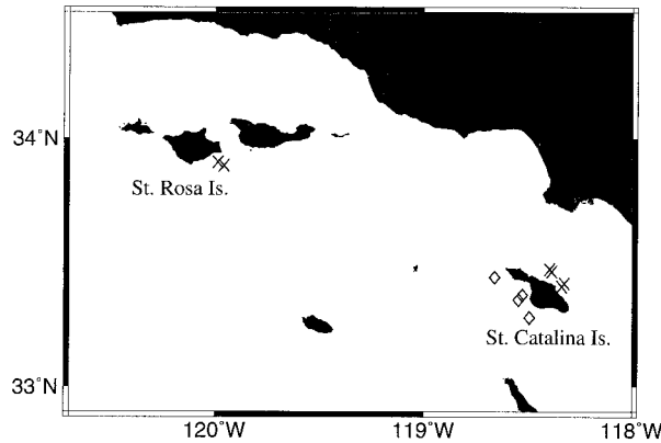
FIG. 2. Location of Coastal Ocean Processes Experiment (CoOP). Crosses, sites with high and variable surface enrichment values. Diamonds, sites with low surface enrichment values.
