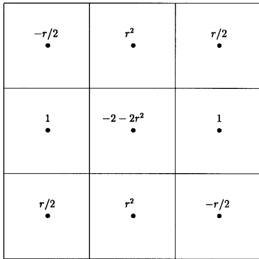
FIG. 2. Stencil for the new method of (Griffies et al. 1997) in the case of constant slopes and grid spacings.
