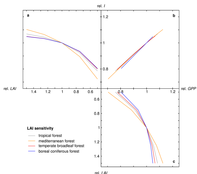
Fig. 3. As in Fig. 1 but varying leaf area index by 25% and 50%.
