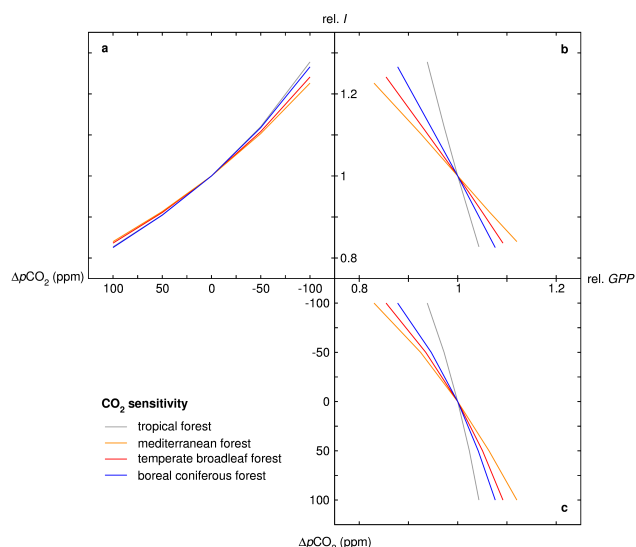
Fig. 2. As in Fig. 1 but varying atmospheric \text{CO}_2 concentration by 50 ppm and 100 ppm.
