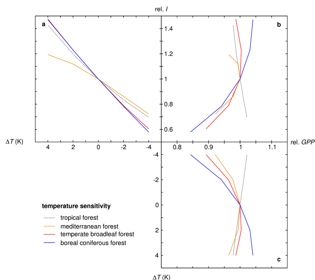
Fig. 1. Response of canopy isoprene emissions ( I ) to a change in temperature ( \Delta T , panel a) and the effects of the corresponding changes in gross primary productivity (GPP) on I (panel b), and the interactions of GPP and T (panel c). The distribution of plant functional types, climate and \text{CO}_2 concentration were prescribed using the average of the years 1981–2002 (obtained from standard model runs as in e.g., Arneth et al (2007a)), and temperature was decreased and increased by 2 K and 4 K on an annual basis. I and GPP are expressed relative (rel) to their 1981–2002 averages, while \Delta T is the difference to the average T over this period. The difference between the temperature optimum of photosynthesis and isoprene emissions is accounted for as described in Arneth et al. (2007b). The y-axis of panels a and b denotes rel I in response the changes in T and GPP, the x-axis of panels c and b shows rel GPP. Locations are:
