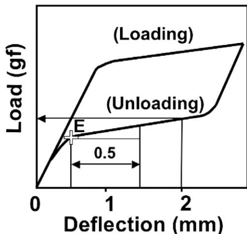
Figure 2. Evaluation points for load-deflection curve.
