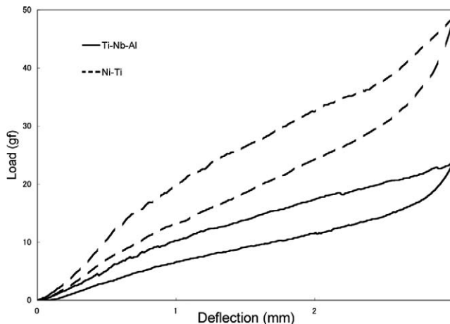
Figure 3. Load-deflection curves for titanium-niobium-aluminum and nickel-titanium expansion springs.
