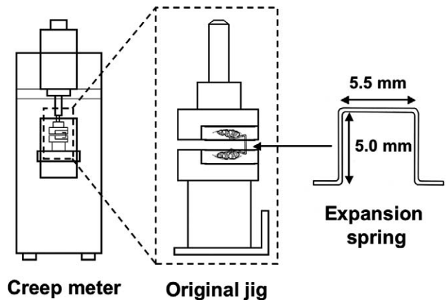
Figure 1. Schematic view of standardized expansion spring and load-deflection measurement with original jig.
