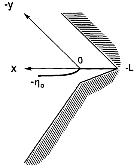
FIG. 1. A semi-infinite, straight shelf-slope region.
