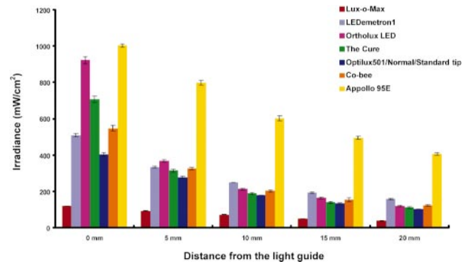
FIGURE 2. The light intensity measured with the curing radiometer at the defined distance.
